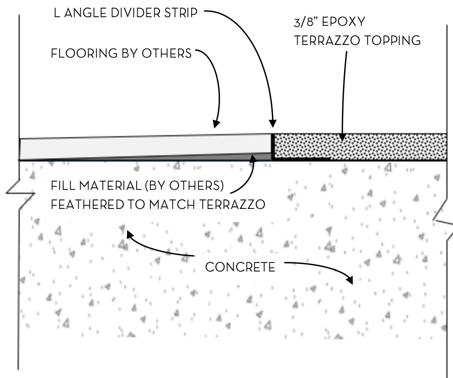
Feathered Ramp Transition
