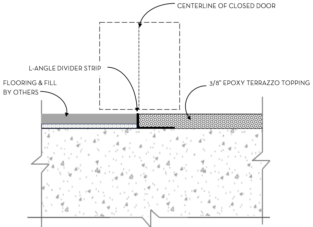
Divider Strip @ Door with Other Floor Finish
